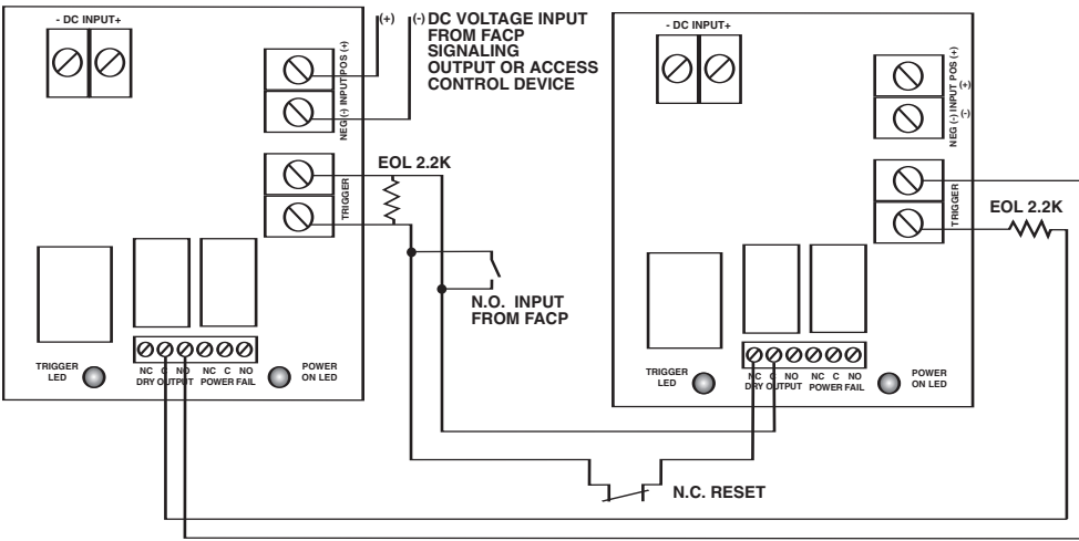
Fig. 6 - Two (2) MOM5C modules shown with wet and/or dry normally open fire alarm trigger inputs ( Latching with Manual Reset ):
