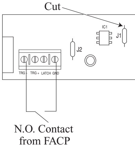
Fig. 4 FireSwitch16D module shown with N.O. Dry trigger.
