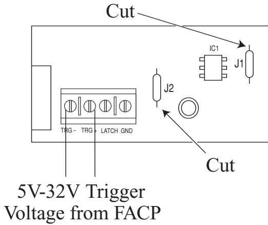
Fig. 2 FireSwitch16D module shown with wet voltage trigger.
